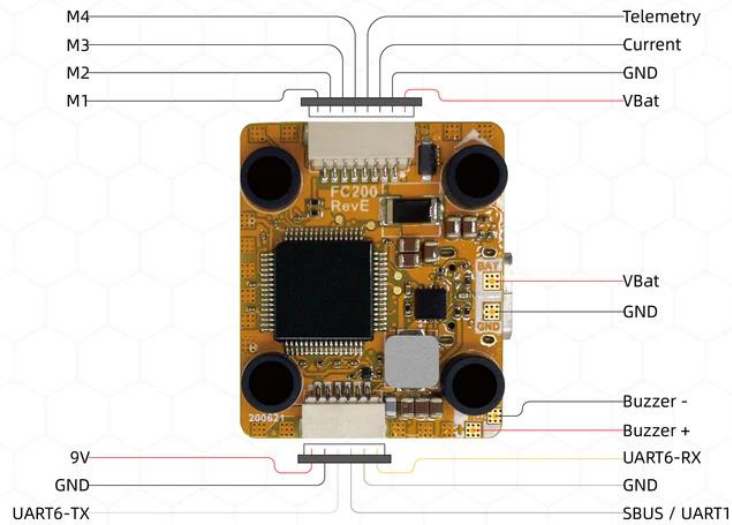
Infinity200 F4 Flight Controller
